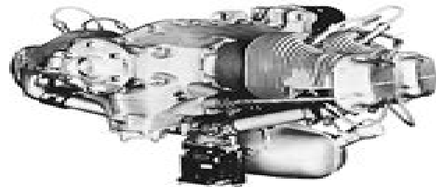
Figure 3. Three-Quarter Left Front View, Model C90-16P.
